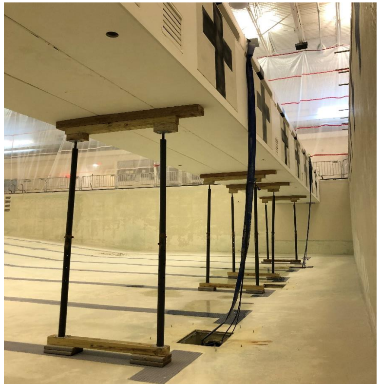
Bracing for Bulkhead
